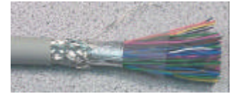
25 Conductor Shielded
